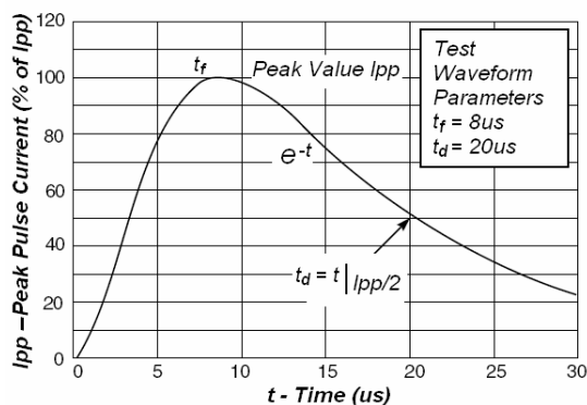
Fig 1. Pulse Waveform
